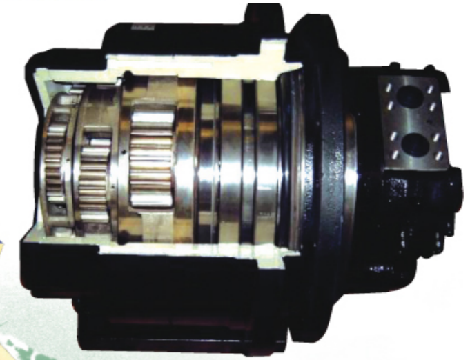
Traveling Reduction Gear Assembly
