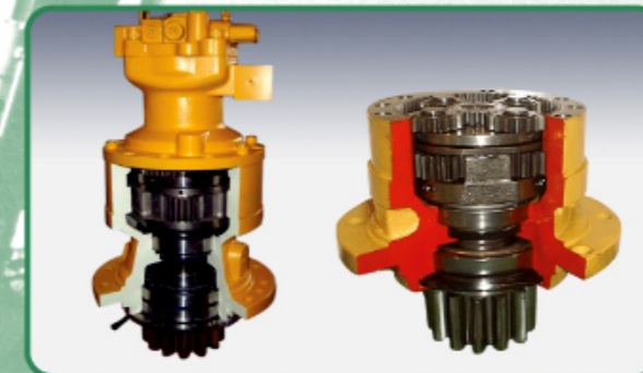
Swing Reduction Gear
